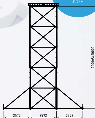
Front view Scale 1:75
